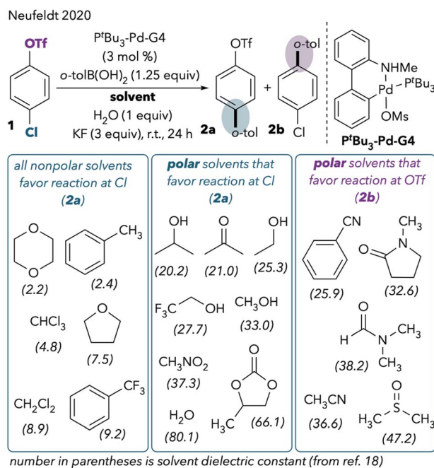
Scheme 2 Expanded solvent effect studies in the Pd/P t Bu 3 -catalyzed Suzuki coupling. 11
