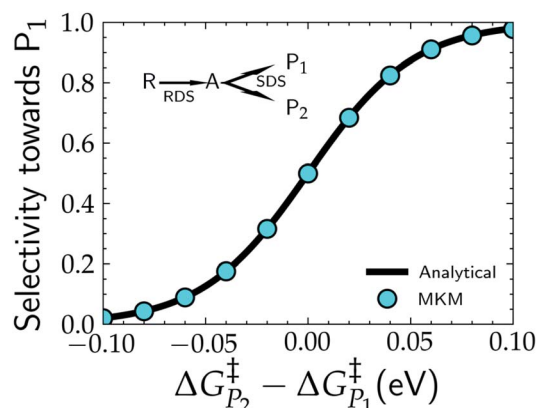
Fig. 4 Selectivity predictions in a model reaction network consisting of a rate determining step (RDS) followed by a selectivity determining step (SDS) leading to the two products, P 1 and P 2 . Cyan points show the results in the selectivity towards P 1 ( S P 1 ) resulting from a microkinetic model (MKM), with S P 1 calculated via eqn (8), while the solid black line represents the same selectivity calculated from the analytical eqn (9).
