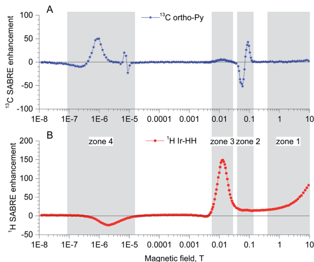
Fig. 9 (A) ^{13}\text{C} SABRE field dependence for ortho carbon of ^{15}\text{N} -pyridine, for details see ref. 142. (B) ^1\text{H} SABRE field dependence for hydride protons on Ir-catalyst (unpublished results provided by A. Kiryutin).
