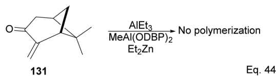
Scheme 38 Lewis acid ( \text{AlEt}_3 )-assisted polymerization of pinacarvone.
