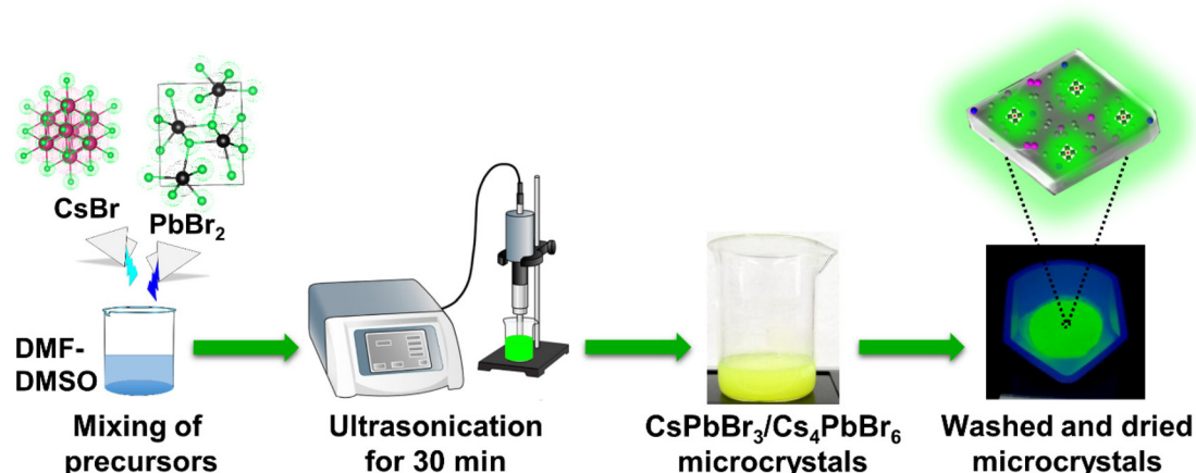
Fig. 1 Scheme for the synthesis of dual-phase \text{CsPbBr}_3/\text{Cs}_4\text{PbBr}_6 MCs using ultrasonication process.
