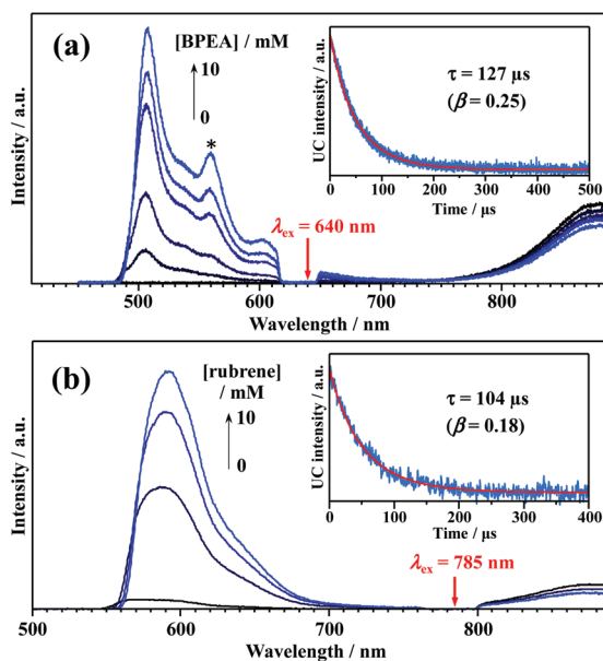
Fig. 3 PL emission spectra of (a) Au_{25} -rod (13 \mu M)/BPEA (0–10 mM) excited at 640 nm ( 10 \text{ W cm}^{-2} ) and (b) Au_{25} -rod (40 \mu M)/rubrene (0–10 mM) excited at 785 nm ( 5.5 \text{ W cm}^{-2} ) in deaerated THF. The asterisked peak in panel (a) begins to appear when the BPEA concentration exceeds \sim 5 mM and is assigned to the emission from BPEA aggregates (Fig. S4a † ). Insets in panels (a and b) show the decay curves obtained by monitoring only the upconverted emission from BPEA and rubrene, respectively.
