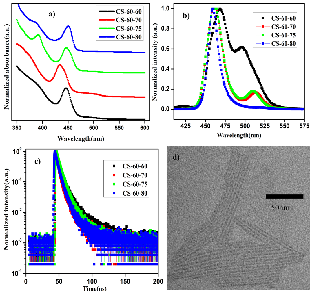
Fig. 3 (a) UV-visible absorption and (b) normalized PL emission spectra of the NPLs synthesized at 60 °C with different PbBr 2 precursor temperatures. (c) TRPL decay curves for the NPLs synthesized at 60 °C under different conditions. (d) TEM image of the sample CS-60-80.
