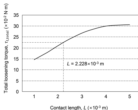
Fig. 11 The effect of contact length, L , on the total loosening torque, \tau_{l,total} . This graph shows total loosening torque values, based on the data in Table 1.
