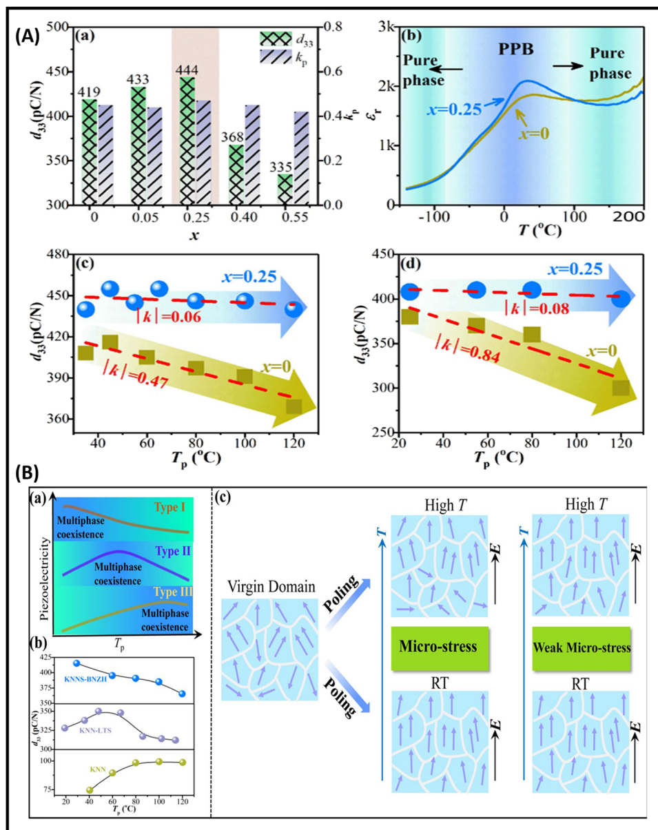
Fig. 7 (A) Compositional and temperature dependence of piezoelectric properties: (a) fluctuation of d_{33} and k_p values with heavy metal content ( x = 0-0.55 ); (b) variation of \epsilon_r with composition ( x = 0-0.25 ) and T_p = -150 to 200 °C; and (c) and (d) variation of d_{33} with T_p with DC (c) and AC (d) poling with x ( 0-0.25 ). (B) (a) Dependence of d_{33} with T_p for KNN-based materials, (b) plots of d_{33} with respect to T_p for various KNN-based ceramics, 90,91 and (c) schematic of domain behaviour with poling temperature and field; reproduced with the permission from ref. 89. Copyright Wiley publications.
