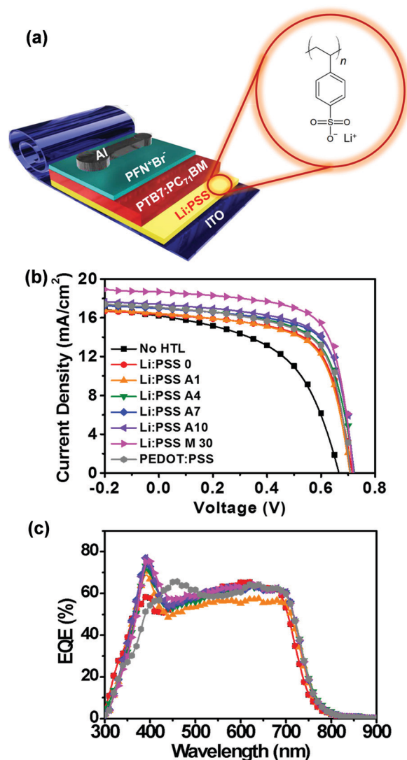
Fig. 2 (a) Device architecture of conventional OSCs with ITO/Li:PSS/PTB7:PC 71 BM/PFN + Br - /Al and the chemical structure of Li:PSS, (b) J - V curves of PTB7:PC 71 BM OSCs measured under simulated AM 1.5G solar light and (c) EQE spectra.
