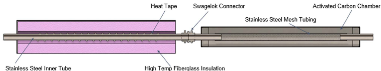
Fig. 2 Cross-sectional view of the thermodenuder used in the study, highlighting its different components. The temperature of the heating section was monitored via a K-type thermocouple placed at the mid-section surface of the sampling tube, providing feedback to an external temperature controller unit. The aerosol flow direction is from the left towards the denuder section to the right.
