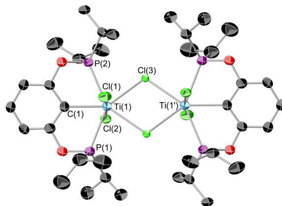
Fig. 5 ORTEP plot of 4 . Thermal ellipsoids at 50% probability, hydrogens omitted for clarity. Selected bond lengths (Å) and bond angles (°): Ti(1)-Cl(1) 2.293(1), Ti(1)-Cl(2) 2.336(1), Ti(1)-Cl(3) 2.587(1), Ti(1)-P(1) 2.578(1), Ti(1)-P(2) 2.587(1), Ti(1)-C(1) 2.252(4), Ti(1)-Ti(1') 4.116(1), \Sigma equatorial angles 360.89(5), Cl(1)-Ti(1)-Cl(2) 174.05(5).
