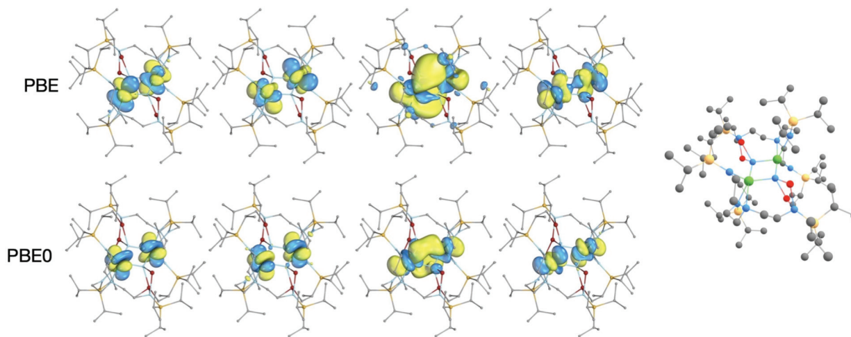
Fig. 4 Singly-occupied \alpha -spin Kohn Sham MOs of the {}^5A_g ground state of 2-opt (top: PBE, bottom PBE0). The isosurfaces enclose 90% of the orbitals. Hydrogen atoms are omitted for clarity. The ball and stick representation of 2-opt is shown to provide orientation of the molecular orbital representations.
