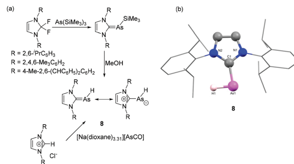
Fig. 4 (a) Synthesis of NHC-arsinidene 8 starting from [AsCO] – and As(TMS) 3 ; (b) solid-state structure of 8 .
