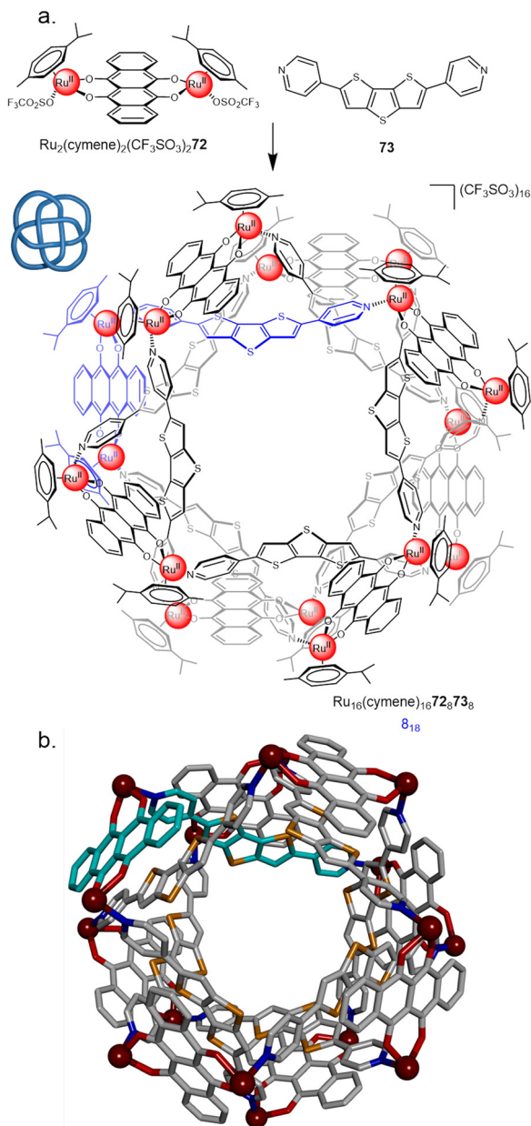
Fig. 25 (a) Synthesis of 8_{18} metalla-knot \text{Ru}_{16}(\text{p-cymene})_{16} \mathbf{72} \mathbf{73} \mathbf{8} . (b) X-ray crystal structure of the 8_{18} metalla-knot with p -cymene ligands omitted for clarity. 100
