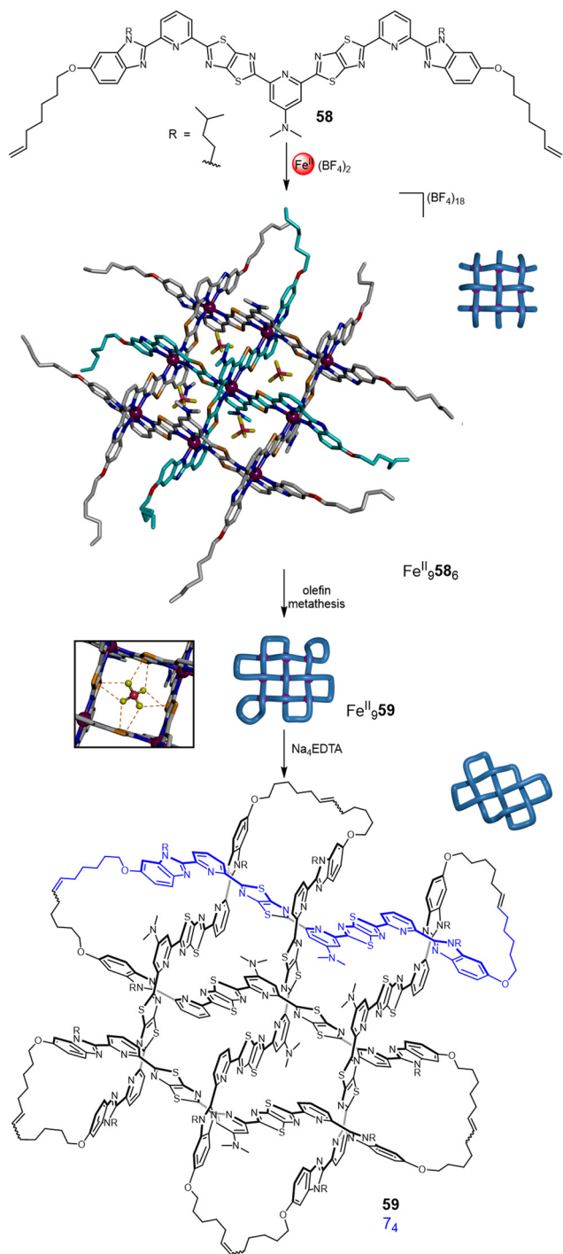
Fig. 21 Weaving molecular endless (7 4 ) knot 59 by self-assembly of an interwoven 3 × 3 grid. 16 Inset: The stabilising effect of the \text{BF}_4^- anions through B–F... \pi and electrostatic interactions.
