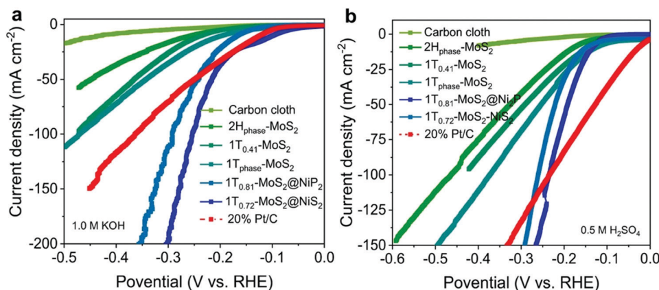
Fig. 83 The electrocatalytic HER performance of 1T_{0.72} -MoS 2 @NiS 2 and 1T_{0.81} -MoS 2 @Ni 2 P hybrid materials in comparison with MoS 2 , carbon cloth and Pt/C. (a) LSV curves in 1 M KOH. (b) LSV curves in 0.5 M H 2 SO 4 . Reproduced with permission from ref. 1185 Copyright Nature Publishing 2021.
