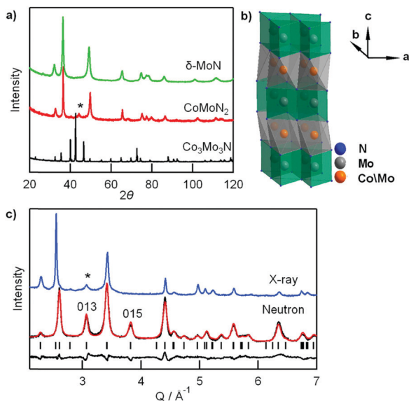
Fig. 67 (a) Lab X-ray powder diffraction patterns of \delta -MoN, \text{CoMoN}_2 , and \text{Co}_3\text{Mo}_3\text{N} . Asterisk marks the impurity peak of cobalt metal. (b) Four-layered crystal structure of \text{CoMoN}_2 . (c) Rietveld refinements of neutron diffraction for \text{CoMoN}_2 showing observed data (black line), calculated pattern (red line) and difference curve (bottom line). Lab X-ray diffraction data (blue line) in same Q ( = 2\pi/d ) range between 2 and 7 \text{ \AA}^{-1} do not clearly show superstructure peaks such as the 013 and 015 reflections which are intense in neutron diffraction data. Reproduced with permission from ref. 1030. Copyright American Chemical Society 2013.
