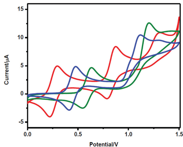
Fig. 131 Water oxidation in the presence of \text{Co}(\text{tpc})\text{Py}_2 (red), \text{Co}(\text{tdfc})\text{Py}_2 (blue) and \text{Co}(\text{tpfc})\text{Py}_2 (green) in acetonitrile on adding 4.8% water. Reprinted with permission from ref. 1577 Copyright 2020. American Chemical Society.
