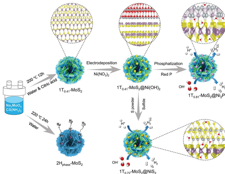
Fig. 82 Schematics of the 1T_{0.72} -MoS 2 @NiS 2 and 1T_{0.81} -MoS 2 @Ni 2 P synthesis steps. Reproduced with permission from ref. 1185 Copyright Nature Publishing 2021.
