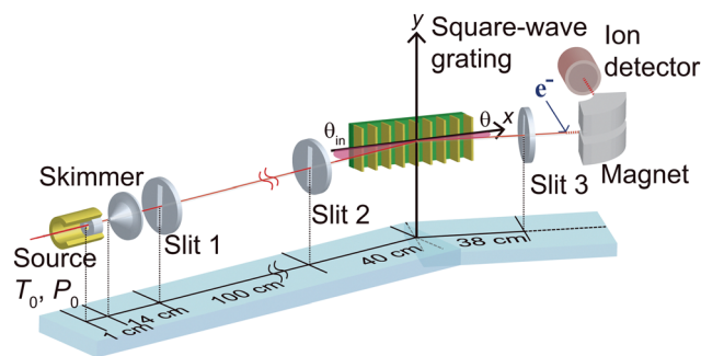
Fig. 2 Schematic of the experimental setup used for reflection of He molecular beams from square-wave gratings. The illustration shows the definitions of the incidence angle \theta_{in} and detection angle \theta .
