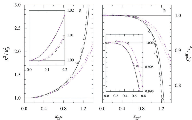
Fig. 18 The ratios (a) \kappa^2 / \kappa_D^2 and (b) \epsilon_r^{\text{eff}} / \epsilon_r plotted as functions of \kappa_D a \sim \sqrt{I} , where I is the ionic strength, for monovalent electrolytes in aqueous solution at room temperature. The inset shows the behaviour at low \kappa_D a . The dot-dashed curves are from the extended exponential DH approximation (EDHX), dotted curves from the Attard's self-consistent screening length approximation (SCSL). 318 The full curves are from the simple multiple-decay extended Debye-Hückel (MDE-DH) approximation, while the dashed curves and crosses show results from HNC calculations, and open circles are from MC simulations. The HNC and MC data are taken from work by Ulander 304 and Ennis. 303 Reproduced from ref. 305 with permission from the Royal Society of Chemistry, copyright 2020.
