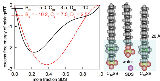
Fig. 15 Dependence of the excess free energy of mixing for surface and micelles on the composition of SDS- C_{12}SB mixtures, and a suggested molecular packing arrangement at the A-W interface. Redrawn from Li et al. 126
