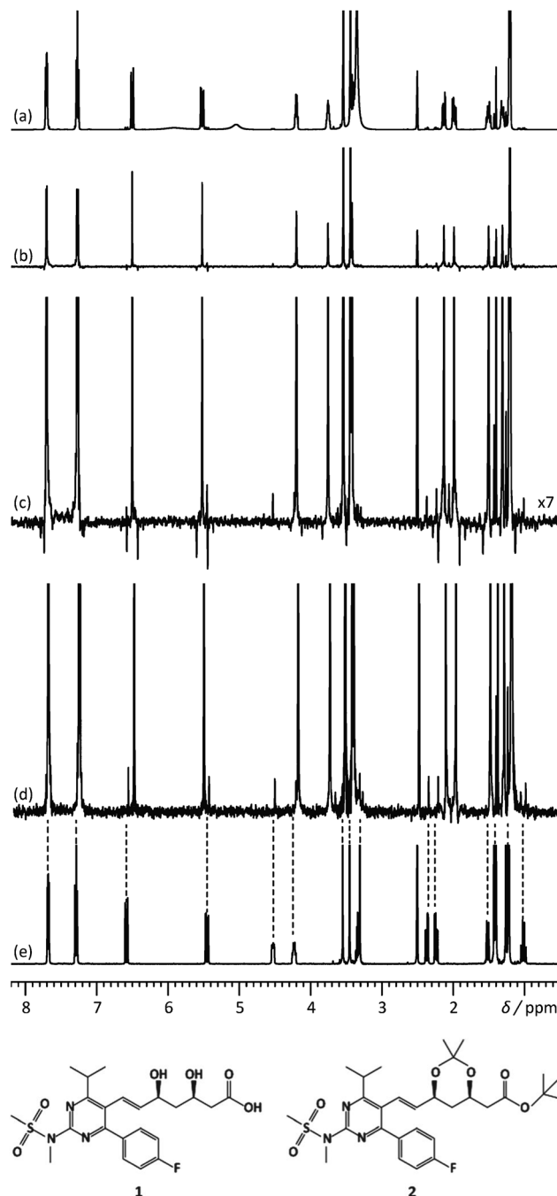
Fig. 2 500 MHz (a) 1D 1 H spectrum, (b) 1 H pure shift spectrum recorded using the unmodified Zangger–Sterk pulse sequence, (c) vertical expansion of the spectrum (b and d) 1 H pure shift spectrum acquired with the pulse sequence modified to remove sidebands, for a mixture containing rosuvastatin (1) and 2.8% of its precursor BEM (2). (e) 1D 1 H spectrum of BEM. Spectra c and d were acquired in approximately 9 h with an sw1 of 39.0625 Hz and 16 chunks using an RSNOb spatially selective spin inversion element with a peak RF amplitude of 47 Hz. Reproduced from ref. 25 with permission from the Royal Society of Chemistry.
