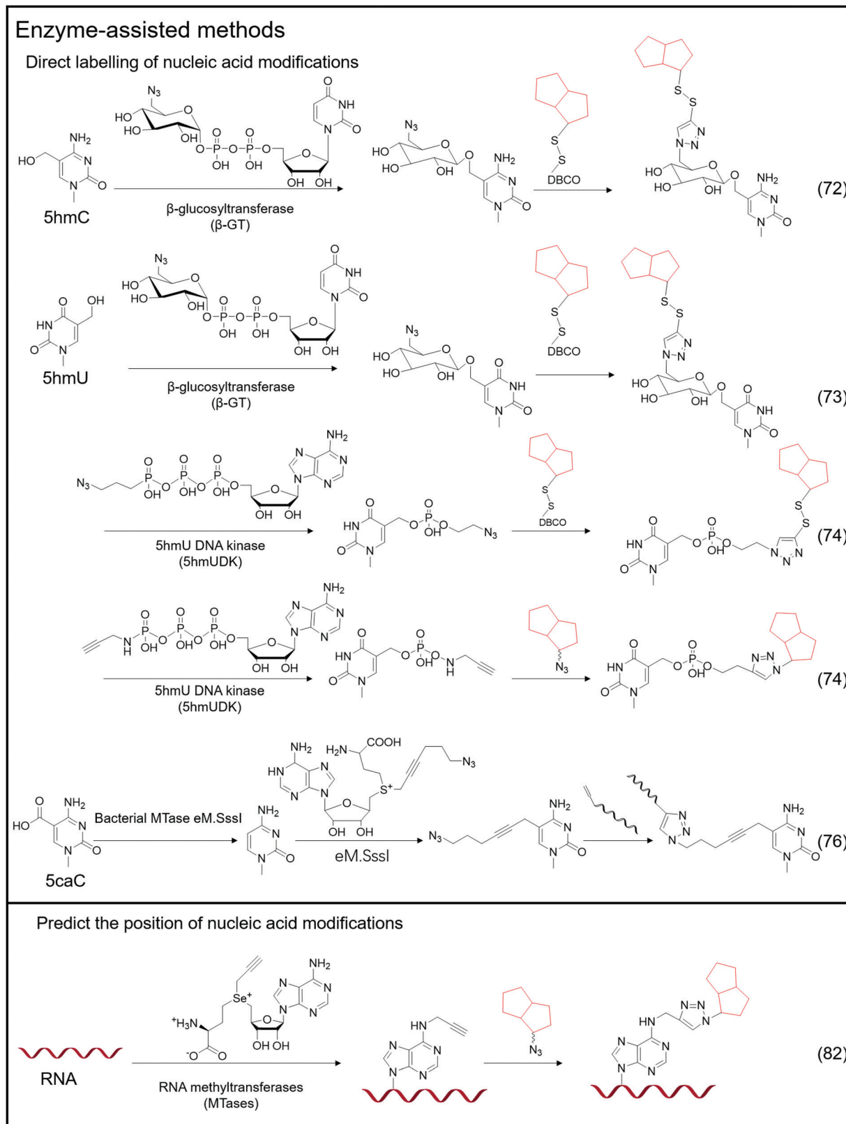
Fig. 5 Enzyme-assisted methods for labelling nucleic acid modifications.
