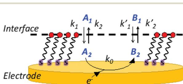
Fig. 3 Schematic representation of the partitioning of reactant A and product B at the interface solution/modified electrode.
