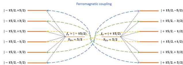
Fig. 14 Energy splitting of the lowest manifold arising from the exchange coupling between a strong anisotropic lanthanide ion (e.g., \text{Dy}^{\text{III}} ) and a transition metal ion (e.g., \text{Fe}^{\text{III}} ) in weak ZFS. Here orange lines are energy levels, colored lines with arrows indicates the most preferred relaxation channel for population at corresponding energy level. Lines with the same color are expected to have the same transition rate. Dominant path is the competition between different colored lines. Effective blocking barrier can thus range from the height of the fourth to the sixth energy levels depending on the specific system and temperature.
