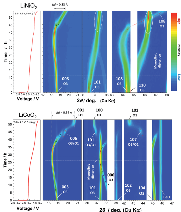
Fig. 2 Contour plots for selected ranges obtained from the in situ XRD patterns of \text{LiNiO}_2 and \text{LiCoO}_2 at a rate of 5 mA g -1 , and corresponding initial charge curves in electrochemical cells are also shown. The original in situ XRD data are shown in ESI Fig. S3.†
