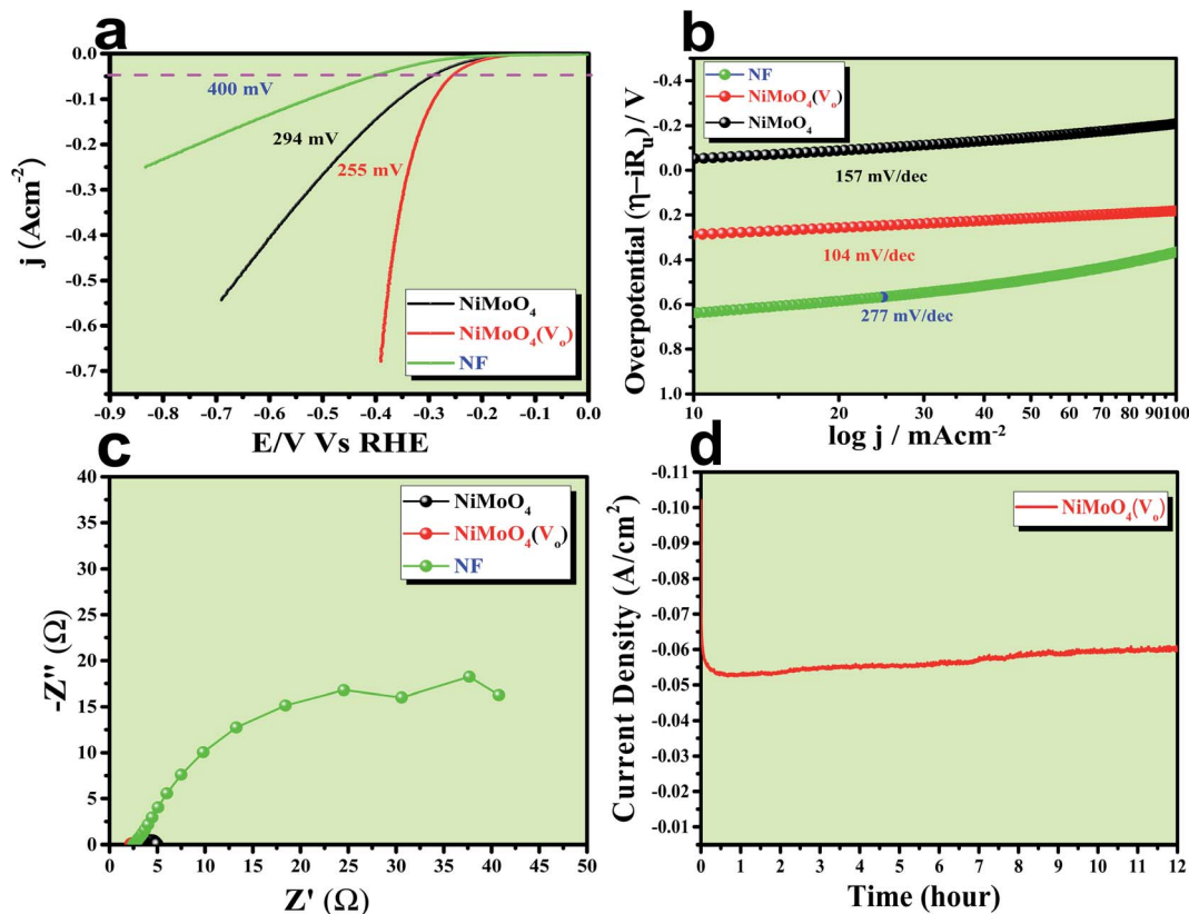
Fig. 9 (a) LSV curve of rod like \text{NiMoO}_4(\text{V}_o) and \text{NiMoO}_4 at a scan rate of 5 \text{ mV s}^{-1} , (b) corresponding Tafel plot, (c) impedance spectra obtained at 250 \text{ mV} overpotential and (d) chronoamperometric outcomes for 12 hours.
