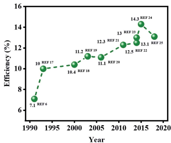
Fig. 1 Evolution of conversion efficiencies of DSSCs in recent years.
