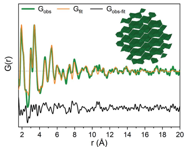
Fig. 8 GaOOH modelled using two GaOOH phases at R = 2.5 for Ga(NO 3 ) 3 solution. The refined structure of the large GaOOH phase is shown as the inset.
