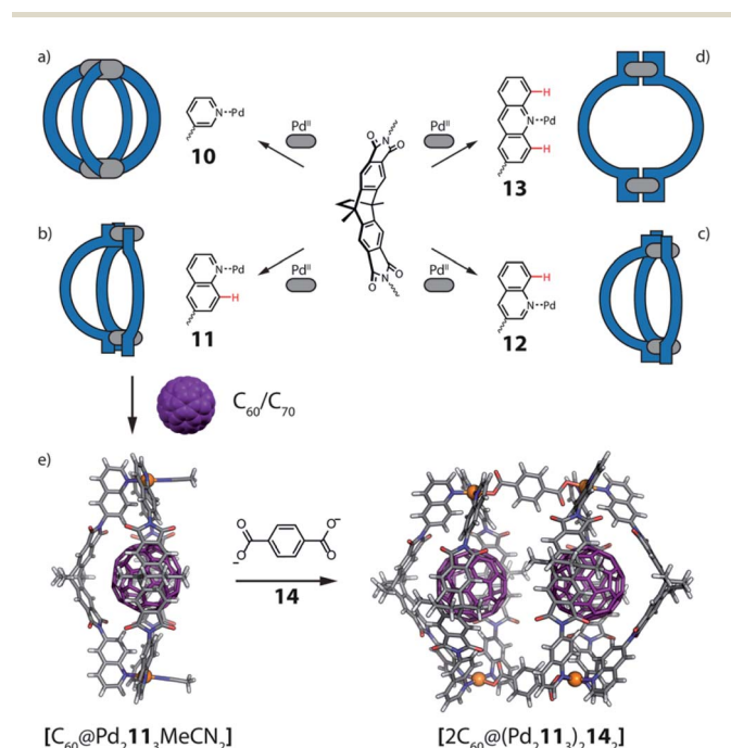
Fig. 7 Formation of (a) cage [\text{Pd}_2\text{L}_4] when using pyridine donors; (b) and (c) [\text{Pd}_2\text{L}_3\text{Solv}_2] bowls when using quinoline donors and (d) a [\text{Pd}_2\text{L}_2\text{Solv}_4] ring using acridine donors. (e) Crystal structure of \text{C}_{60}@[\text{Pd}_2\text{11}_3] bowl and DFT model of heteroleptic, pill-shaped dimer, binding two fullerenes \text{C}_{60} .
