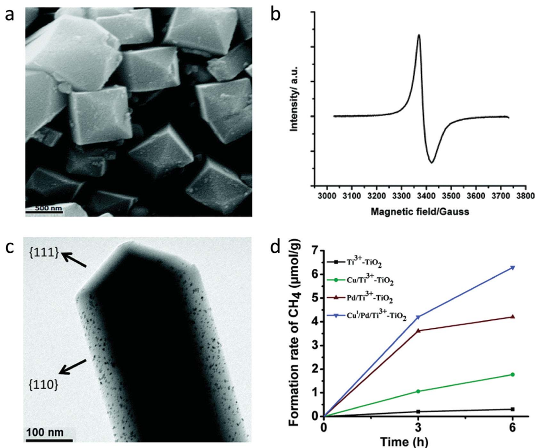
Fig. 19 (a) SEM image of the Ti 3+ -TiO 2 sample and (b) EPR spectra of the Ti 3+ -TiO 2 sample recorded at 100 K, (c) TEM images of the Cu I /Pd/Ti 3+ -TiO 2 sample, and (d) comparison of photocatalytic CO 2 conversion using different samples (reproduced from ref. 73 with permission from the Royal Society of Chemistry, copyright 2015).
