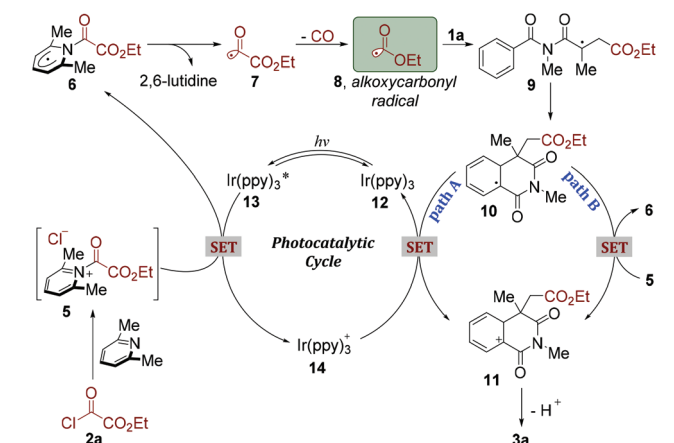
Scheme 2 Proposed mechanism.
