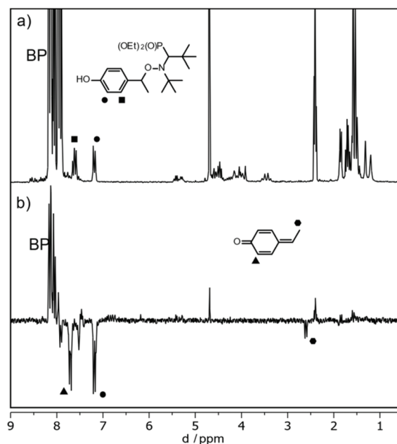
Fig. 6 ^1\text{H} NMR (a) and (b) CIDNP spectrum of 3a and BP in Acetonitrile- d_3 / \text{D}_2\text{O} recorded 2 \mu\text{s} after the laser flash (355 nm, 8 ns).
