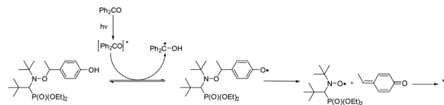
Scheme 5 generation of 3' during the irradiation (NdYAG laser, 355 nm, 8 ns) of benzophenone (3 mM) in the presence of 3a (1 mM) at 25 ^\circ\text{C} in acetonitrile- d_3 / \text{D}_2\text{O} .
