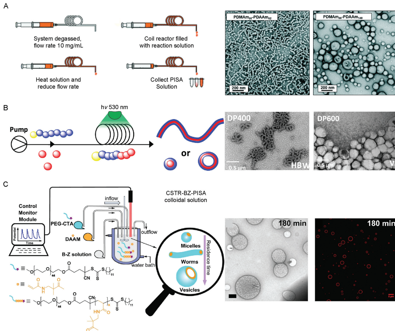
Fig. 4 Methods used to produce vesicles by PISA in flow by (A) thermal-initiated RAFT polymerization of DAAM from PDMAM 50 mCTA. Adapted with permission from ref. 84. Copyright 2019 Royal Society of Chemistry. (B) Photo-initiated PET-RAFT of diacetone- stat -dimethyl acrylamide from a PDMA trithiocarbonate mCTA. Reproduced with permission from ref. 86. Copyright 2019 American Chemical Society. (C) BZ-initiated PISA of DAAM from a PEG 44 trithiocarbonate mCTA using a CSTR in flow. Scale bar = 500 nm (TEM image) and 5 μm (fluorescence image). Reproduced with permission from ref. 29. Copyright 2019 Springer Nature.
