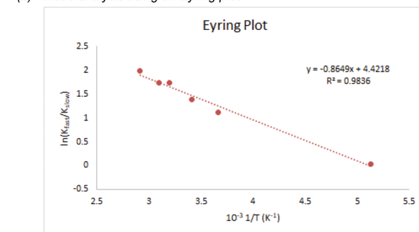
(b) Kinetic analysis using an Eyring plot
