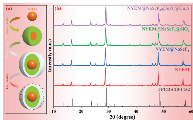
Fig. 1 (a) A description of the preparation of \text{NYEM}@/\text{NaScF}_4/\text{SiO}_2/\text{Cu}_2\text{S} . (b) XRD diffraction patterns of the samples synthesized at various steps along with the reference data of hexagonal \text{NaScF}_4 (JCPDS 20-1152).
