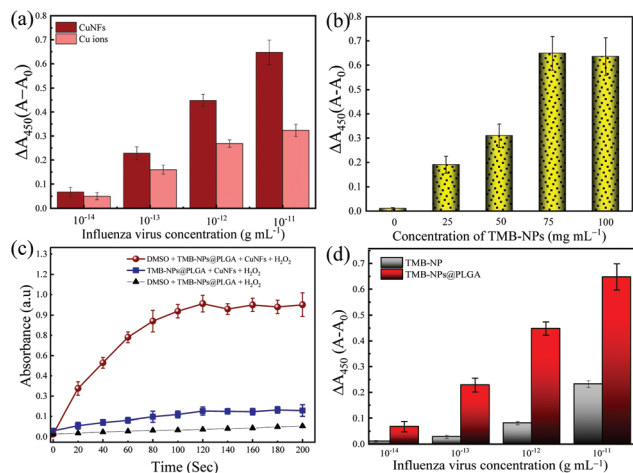
Fig. 3 (a) Comparison of the catalytic activity of CuNFs and Cu ions in the \text{H}_2\text{O}_2/\text{TMB} system for various concentrations of IV; the optimization of the TMB-NPs@PLGA corresponding to the encapsulation amounts of TMB-NPs in PLGA nanovesicles (b) and the incubation time for the change in absorbance intensity of the TMB-NP, CuNF, and \text{H}_2\text{O}_2 mixture (c); (d) comparison of IV/A detection using TMB-NPs@PLGA and TMB-NPs. A_0 and A indicate the absorbance before and after the addition of DMSO, respectively. The error bars indicate the SD of the triple measurement.
