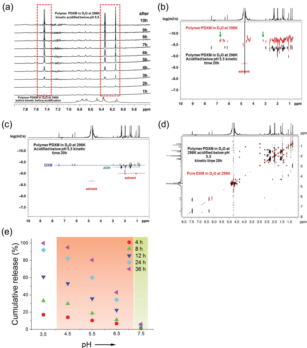
Fig. 3 (a) ^1\text{H} NMR (850 MHz at 298 K) in situ kinetic study of the degradation of PDXM in acidic condition. (b) Overlay of NMR DOSY spectra of PDXM7k polymer (red) and the degradation products in \text{D}_2\text{O} after acidifying at kinetic time of 20 h (black). Green arrows point out the new peaks appearing after polymerization and disappearing after degradation. (c) NMR DOSY spectra of the degradation products of PDXM7k at kinetic time of 20 h. (d) Overlay of NMR COSY spectrum of the degradation products of PDXM7k at kinetic time of 20 h (black) with the spectrum of pure DXM monomer (red). (e) pH-dependency of the degradation and release of PDXM7k. The red background covers the range of pH values in different acidic extra- and intracellular environments reported in the literature. 1,2 The green background represents physiological pH values (around 7.4).
