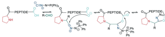
Scheme 41 Multicomponent reaction for peptide macrocyclization employing an aldehyde and ( N -isocyanimino)triphenylphosphorane to form a 1,3,4-oxadiazole.
