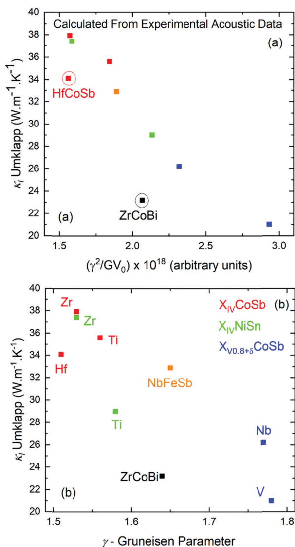
Fig. 3 Plots of calculated lattice thermal conductivity ( \kappa_l ) at 300 K (see Section 2.4), assuming the presence of only Umklapp scattering ( i.e. for the defect free parent materials), versus (a) the variables determining the magnitude of Umklapp scattering and (b) the acoustic Grüneisen parameter. HfCoSb and ZrCoBi have lower \kappa_l due to low \nu_s (see Table 2).
