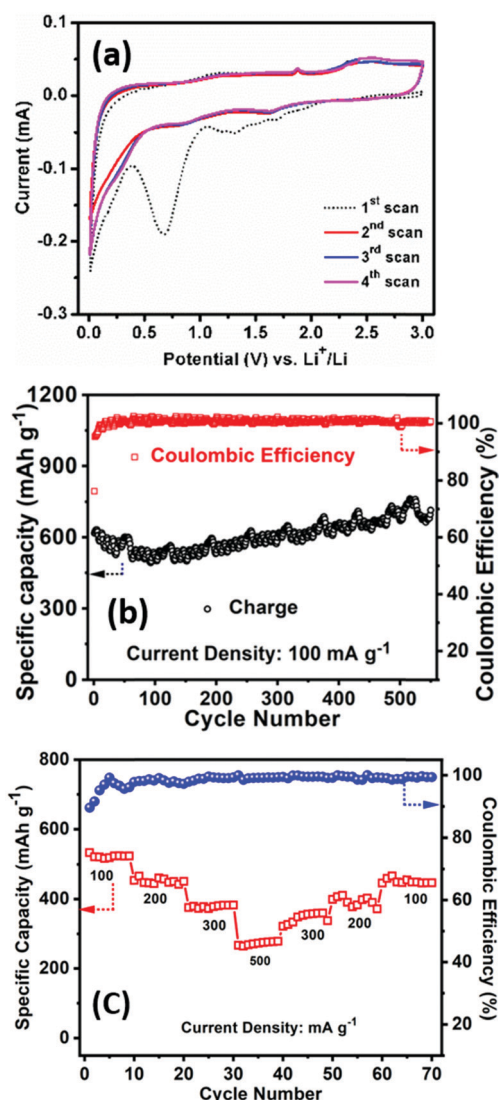
Fig. 5 Electrochemical half-cell LIB anode performance of the PSCNs. (a) Cyclic voltammetry of the PSCN electrode for the first four cycles at 0.1 \text{ mV s}^{-1} at 0.01–3.0 V, (b) cycling performance at 100 \text{ mA g}^{-1} current density, and (c) rate performance at different current densities ( 100\text{--}500 \text{ mA g}^{-1} ).
