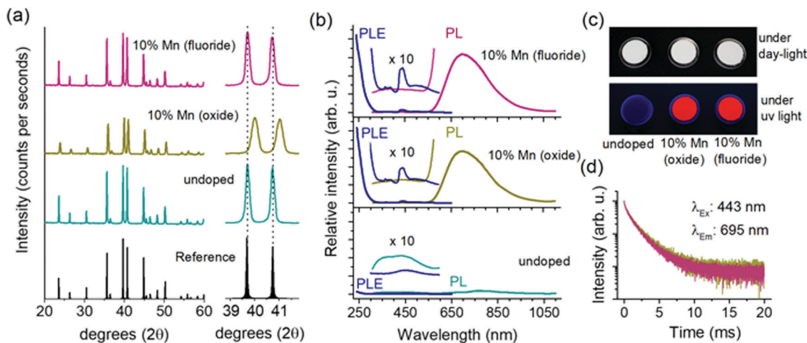
Fig. 2 PXR D patterns of undoped and Mn 2+ (10 at%) doped Ca- \alpha -SiAlON obtained using oxide and fluoride doping precursors (a); respective PL–PLE spectra (b); the photographic images (powders filled in quartz disks) under day-light and UV-light (254 nm Hg vapor lamp) exposure (c); and the Mn 2+ PL decay curves (d). The reference XRD pattern in (a) was calculated for Ca- \alpha -SiAlON structure ( \lambda_{K\alpha} = 1.78897 Å). In (b), the excitation wavelength was 255 nm for PL measurements and the emission was monitored at 695 nm to record the PLE spectra. The insets present enlarged view (10 times) of PL–PLE curves in 300–600 nm range.
