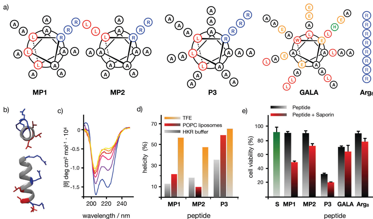
Fig. 1 Peptide structures, helical content quantification by CD and initial screening. (a) Peptides' structures. Sequences: MP1 (Ac-LRLAALARA AAAAAR-NH 2 ); MP2 (Ac-LRAAAAALRA AAAAALR-NH 2 ); P3 (Ac-LRLAALARA AAAAAR AAAAAR-NH 2 ); GALA (Ac-WEAALAEALAEALAEALAEALAEALAEALAA-NH 2 ); Arg 8 (Ac-RRRRRRRR-NH 2 ). (b) 3D prediction of MP1 using PEP-FOLD 3.5. 42 Arginines in blue, leucines in red. (c) Circular dichroism spectra of MP1 (100 µM) at different temperatures (10, 20, 30, 40, 50, 60 °C) in HKR buffer. (d) % helicity of MP1 , MP2 , and P3 in HKR, liposomes (POPC) or TFE at 40 °C (see ESI † ). (e) Cell viability in HeLa cells without (grey) or with (red) 10 µg mL -1 of saporin and 30 µM of the indicated peptides for 1 h and further incubation for 6 h before measuring viability by MTT assay. In green the control with saporin alone. Error bars represent standard deviation (SD) of 3 replicates.
