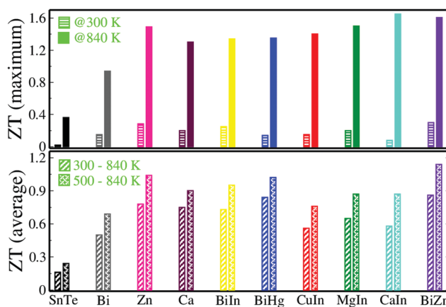
Fig. 6 Comparison of ZT at 300 K and 840 K (upper panel); ZT_{\text{average}} of SnTe and \text{Sn}_{0.92}\text{Bi}_{0.04}\text{Zn}_{0.04}\text{Te} (lower panel) with the reported high performing SnTe based materials. 7–9,11,14,18–20
