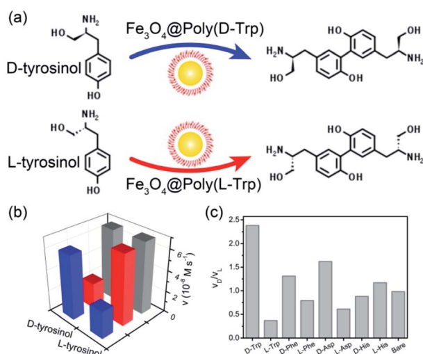
Fig. 2 (a) The enantioselective oxidation of chiral tyrosinol catalyzed by \text{Fe}_3\text{O}_4@ -Poly(L-/D-Trp). (b) The initial velocity for the oxidation of tyrosinol enantiomers with \text{Fe}_3\text{O}_4@ -Poly(D-Trp) (blue), \text{Fe}_3\text{O}_4@ -Poly(L-Trp) (red) and bare \text{Fe}_3\text{O}_4 (gray). (c) The ratio of initial rates for the oxidation of the D enantiomer to L enantiomer.
