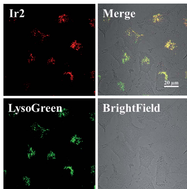
Fig. 2 Intracellular colocalization of Ir2 with the LysoGreen probe observed by confocal microscopy. A549 cells were incubated with Ir2 (10 μM, 4 h) and then stained with LysoGreen (2 μM, 30 min). Scale bar: 20 μm.
