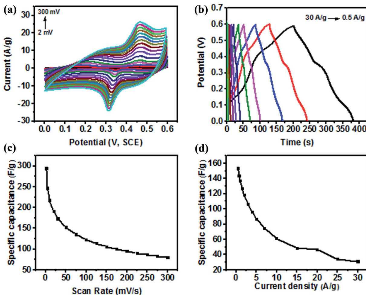
Fig. 8 (a) Cyclic voltammograms of the \text{CoMoO}_4 electrode at various scan rates. (b) Galvanostatic charge–discharge characteristics of \text{CoMoO}_4 at various current densities. (c) Variation of the specific capacitance as a function of the scan rate, and (d) variation of the specific capacitance as a function of the applied current density.
