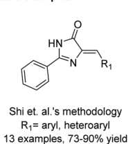
Scheme 23 General transformation of oxazolone to imidazolone.
