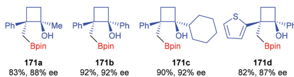
Scheme 48 Asymmetric synthesis of functionalized cyclobutanols via borylcupration.
