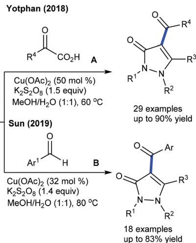
Scheme 141 Synthesis of acyl pyrazolones using aldehydes.
