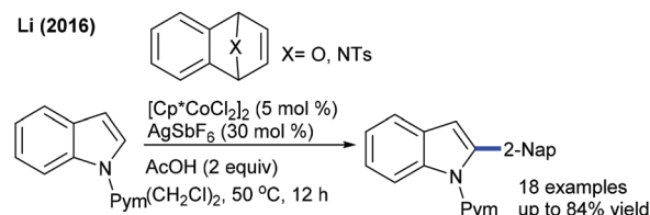
Scheme 21 C2-Naphthylation of indoles.
