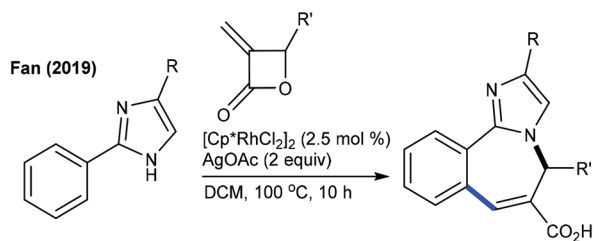
Scheme 83 Annulation of 2-aryl-1 H -imidazoles with methyleneoxetanones.
