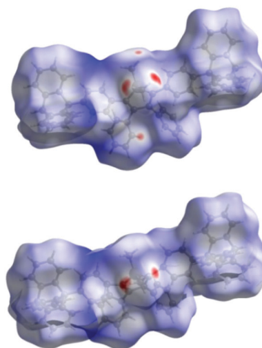
Fig. 5 Hirshfeld surfaces for the L -conformer (top) and the R -conformer (bottom) of Tp-DMTIPS .
