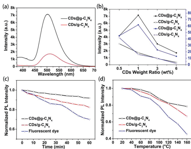
Fig. 5 (a) PL spectra of \text{CDs}@g\text{-C}_3\text{N}_4 and \text{CDs}/g\text{-C}_3\text{N}_4 composites with 1 wt% CD loading concentration under 360 nm excitation. (b) Peak PL intensities under 360 nm excitation of \text{CDs}@g\text{-C}_3\text{N}_4 and \text{CDs}/g\text{-C}_3\text{N}_4 with different CD loading concentrations (black curves) and PLQYs of \text{CDs}@g\text{-C}_3\text{N}_4 and \text{CDs}/g\text{-C}_3\text{N}_4 composites with different CD loading concentrations under 410 nm excitation (blue curves). Evolution of the PL intensities of \text{CDs}@g\text{-C}_3\text{N}_4 , \text{CDs}/g\text{-C}_3\text{N}_4 and organic dye (fluorescein sodium): (c) under UV light exposure ( 1.6\text{ W cm}^{-1} ) and (d) upon heating to 160\text{ }^\circ\text{C} .
